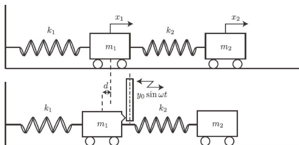
Fig.1 Analytical model of the impact oscillations between a source of external excitation and a main mass coupled with the added oscillatory system. Main mass is subjected to the external excitation source that is pushed against the mass.
