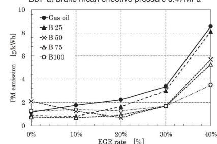
Fig.2 Variations of PM emission with EGR rate measured by using mixed gas oil and BDF fuels (normal operating range within EGR rate 30%)
