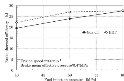
Fig.1 Variations of brake thermal efficiency with fuel injection pressure measured by using gas oil and BDF at brake mean effective pressure 0.47MPa
