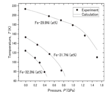
Fig.2 Hydrostatic Pressure dependence of martensitic transformation temperature in Fe-Ni alloys experiment, ---calculation
