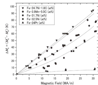
Fig.1 Magnetic Field dependence of martensitic Transformation temperature in Fe-based alloys---calculation
