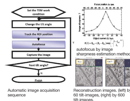
Fig.2 Ultra high voltage electron tomography. Automatic image acquisition sequence with autofocus by image sharpness estimation method, reconstructed tomographic image (bottom right)
