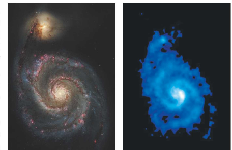
Fig.1 Distribution of stars (left: optical wavelength, Hubble Space Telescope) and molecular gas (right: radio waves, CO(1-0)) Nobeyama 45m radio telescope) in the nearby spiral galaxy M51
