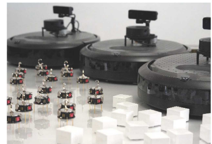
Fig.3 Mobile robots
