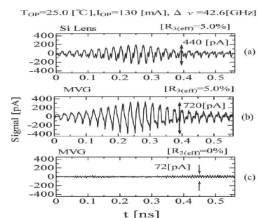
Fig.1 Time series of generated THz waves under the condition of (a)Si lens, R_{3(eff)}=5\% , (b)MVG, R_{3(eff)}=5\% , and (c) MVG, R_{3(eff)}=0\% .
