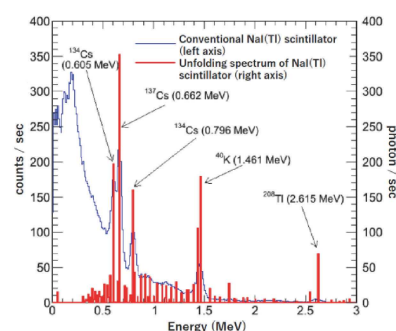
Fig.1 Unfolding spectrum of NaI(Tl) scintillator
