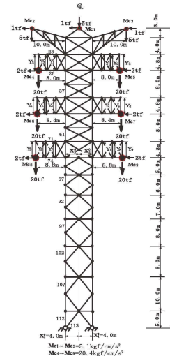
Fig.3 Initial configuration of a transmission tower truss
