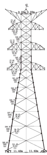
Fig.4 Optimum solution of the truss
