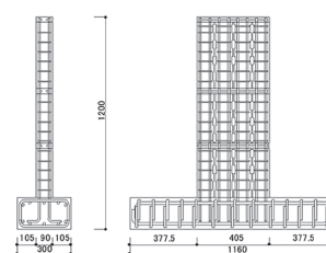
Fig.1 Test specimens
