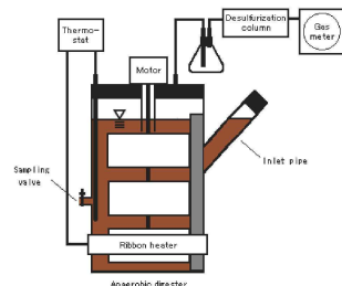
Fig.1 Anaerobic digester system
