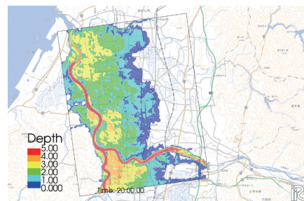
Fig.1 Inundation simulation
